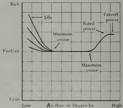
FIGURE 10-39. Idle mixture curve.
